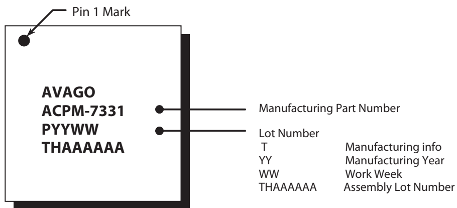
Figure 13. Marking Specifications
